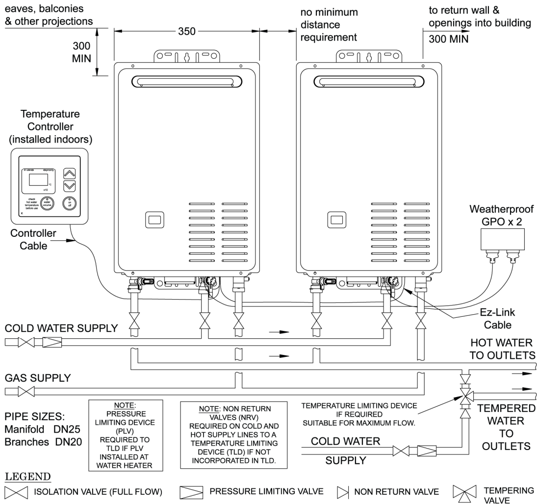
Typical Two Unit Manifold with Ez-Link Connection
