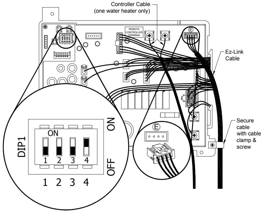
Dip Switch 4 in the on (up) position
